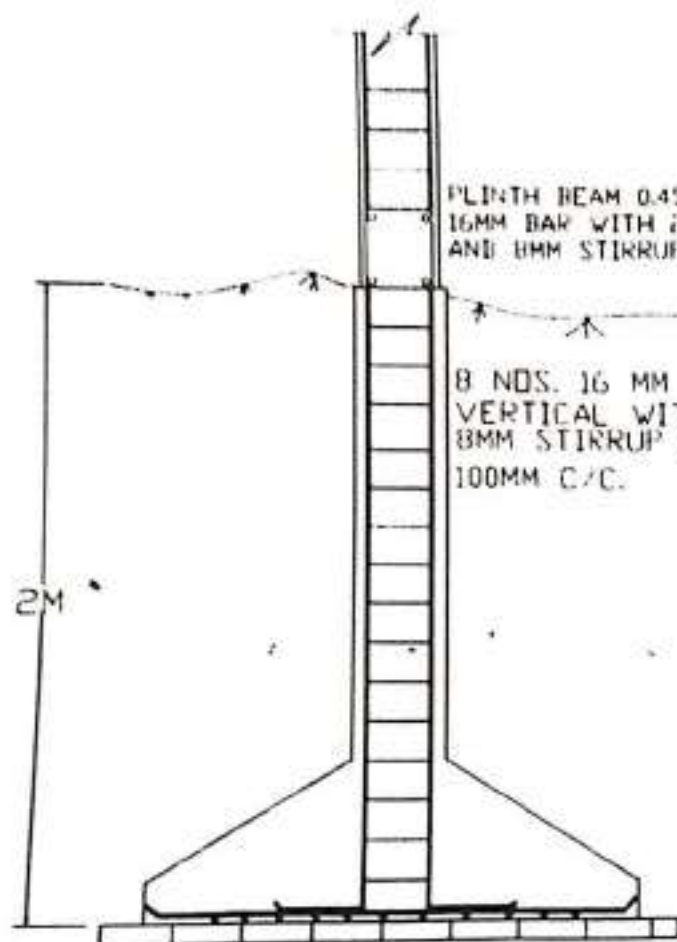
COLUMN SECTION
