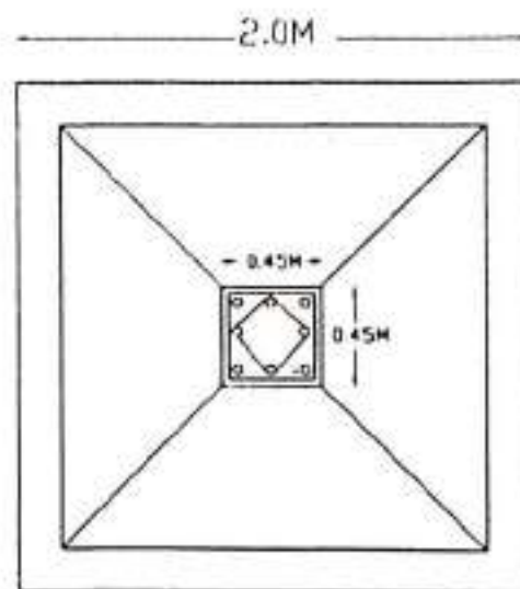
PLAN OF COLUMN
