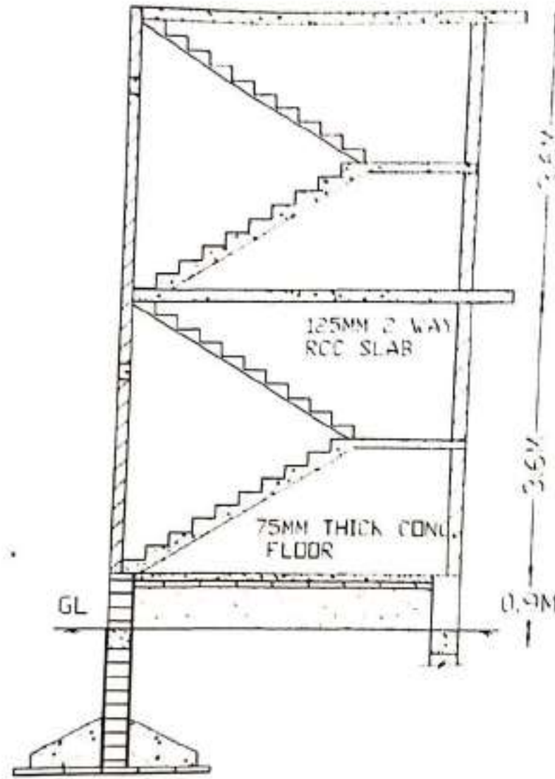
CROSS SECTION
